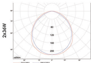
TL240MP-2x36/EVG
